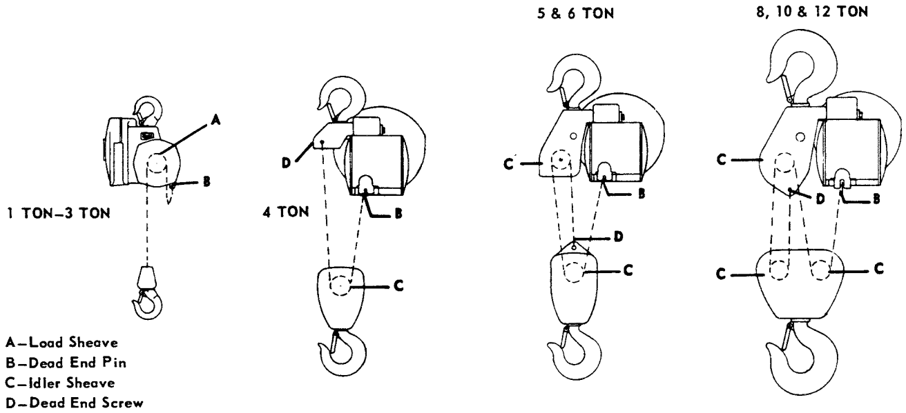
FIGURE 5-4 CHAIN REEVING
