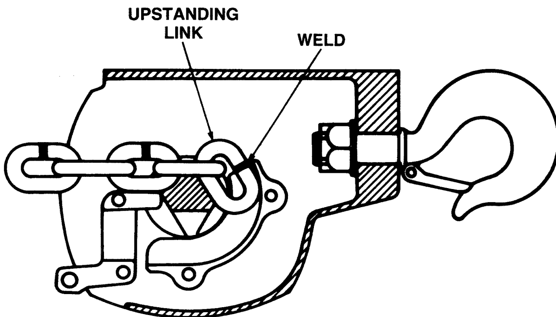
FIGURE 5-2 CHAIN REPLACEMENT
